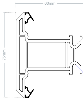
Sash EWS 7055
