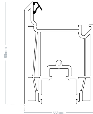
Midrail EWS 7056
